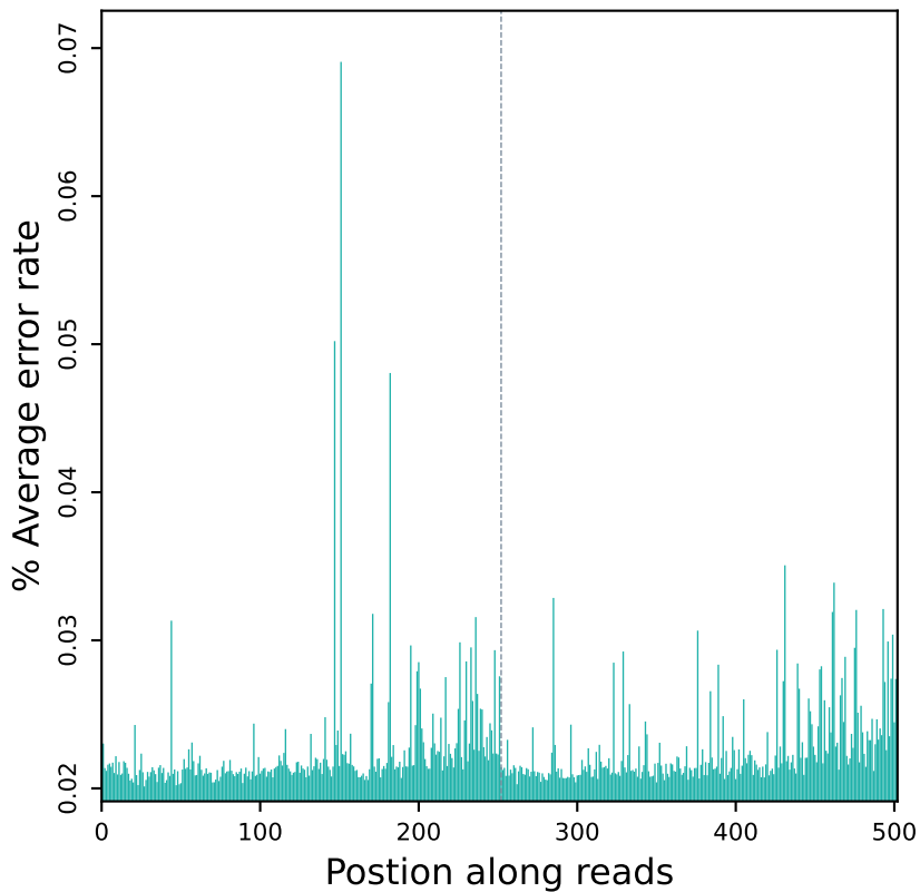
Error rate distribution along reads (R10926)
